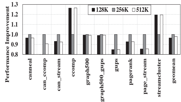
Figure 15: Performance of CSALT with Different Epoch Lengths
