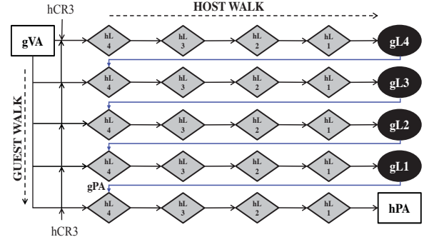
(b) 2-Dimensional Page Table Walk (Virtualized)
